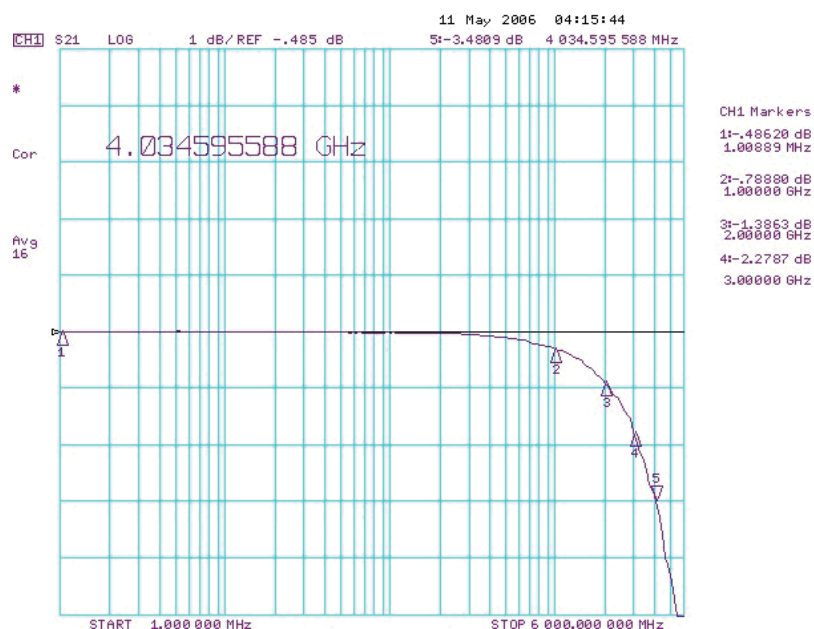
Fig 5: Typical Insertion Loss Plot from 1MHz to 6.0GHz, Vcc=1.8V, 25C
