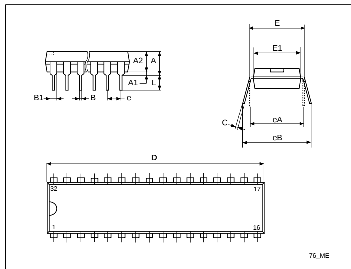
Figure 51: 32-lead shrink plastic DIP (400 ml) package
