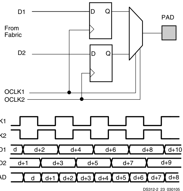
Figure 10: Output DDR
