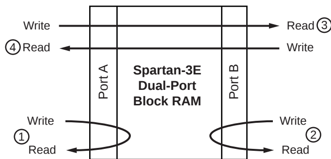
Figure 30: Block RAM Data Paths
