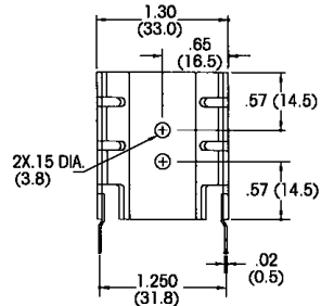
Low Height, Slim Profile Wavesolderable Folded Fin Heat Sinks
