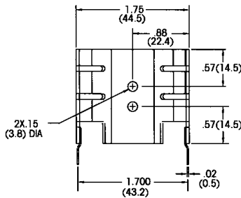
Medium Height, Slim Profile Wavesolderable Folded Fin Heat Sinks
