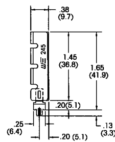
Medium Height, Slim Profile Wavesolderable Folded Fin Heat Sinks
