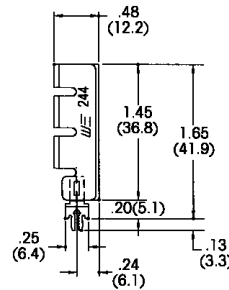
Low Height, Slim Profile Wavesolderable Folded Fin Heat Sinks
