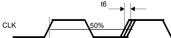
Figure 8. Period Jitter Definition
