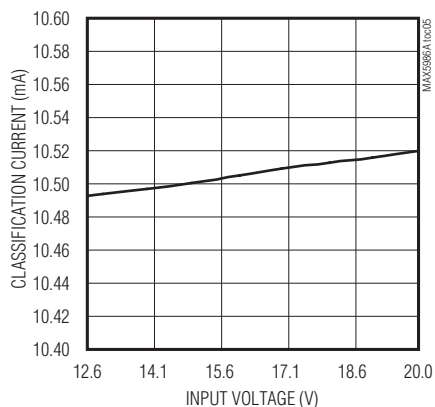
CLASSIFICATION CURRENT vs. INPUT VOLTAGE
