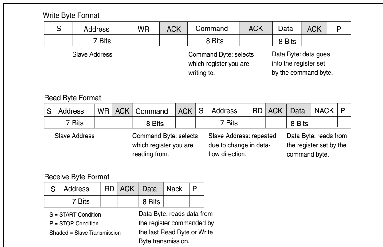
FIGURE 3-1: SMBUS PROTOCOLS
