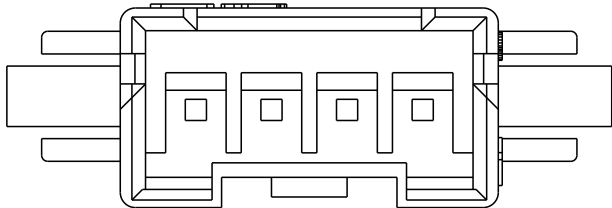
4 POSITION 1969590-4
