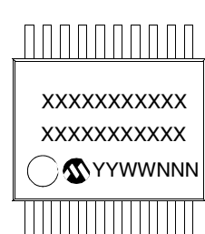
20-Lead SSOP (209 mil, 5.30 mm)
