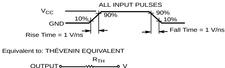
Figure 3. AC Test Loads and Waveforms
