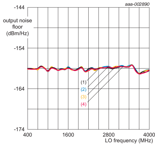
Fig 47. N_{ftr(o)} versus f_{lo} and V_{CC}
