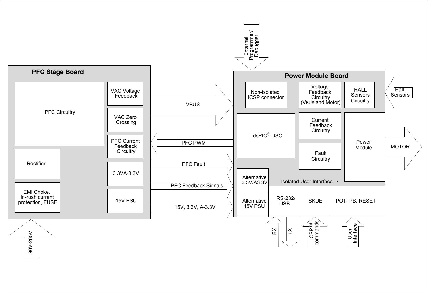
FIGURE 1-2: SYSTEM BLOCK DIAGRAM
