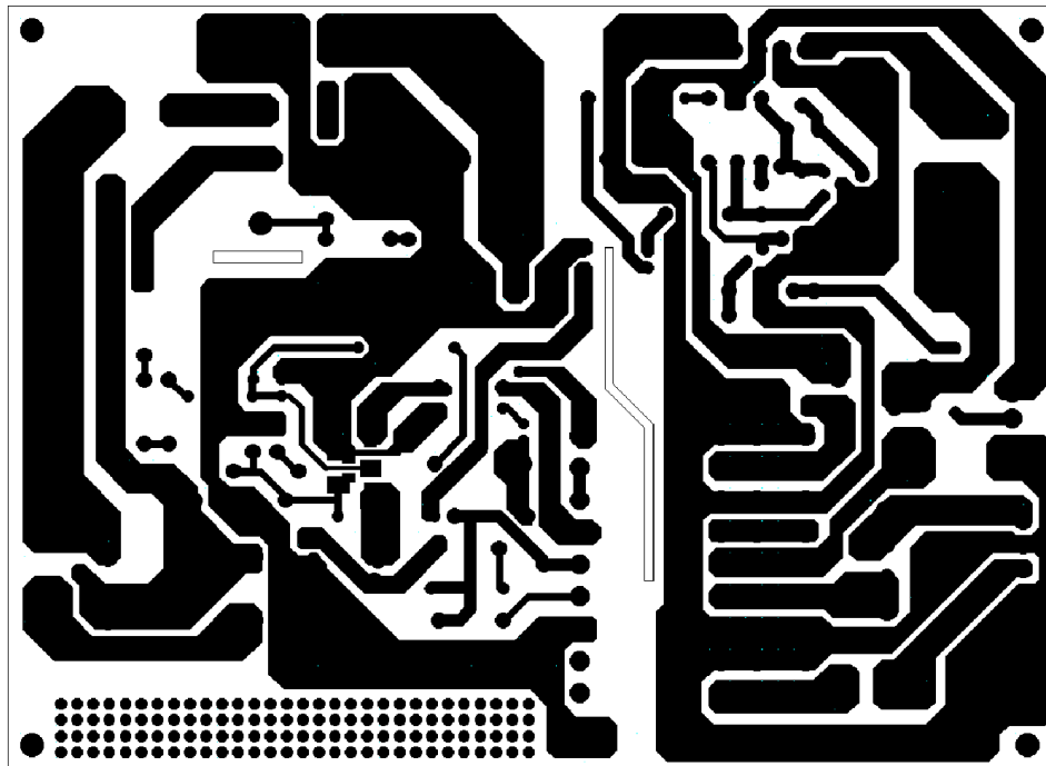
Figure 50. Bottom View
