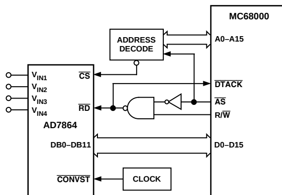
Figure 22. AD7864–MC68000 Interface
