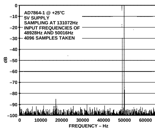
Figure 17. IMD Plot
