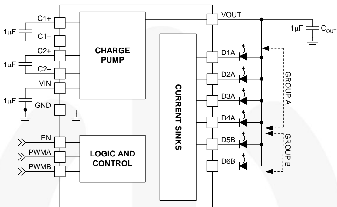
Figure 1. Typical Application
