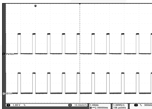
Figure 9. PWM Dimming V_{IN}=3.6V , I_{LED}=20mA , EN=1kHz with 20% Duty Cycle
