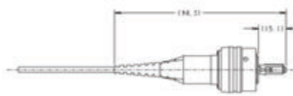
Shown Here: FT/MPO Pigtail Assembly with 4 fiber outdoor ribbon cable
