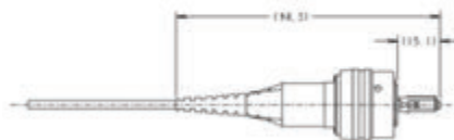
PT/MPO Plug Assembly Shown Here: PT/MPO Pigtail Assembly with 4 fiber outdoor ribbon cable
