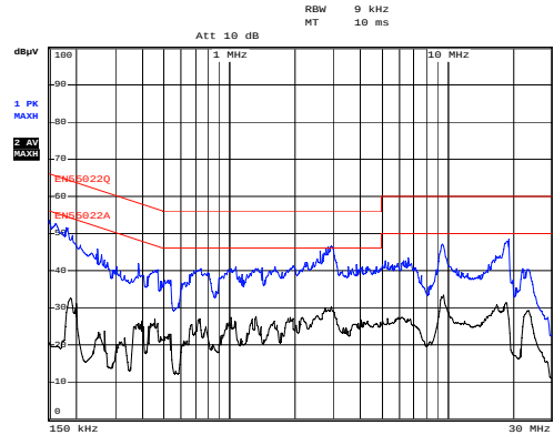
Figure 21. Conduction-Neutral at 230V AC
