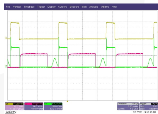
Figure 13. FAN6754AMR+FAN6204MY 230V/50Hz, 80% Load (Ch1: Gate, Ch2: Gate SR , Ch4: V dS )
