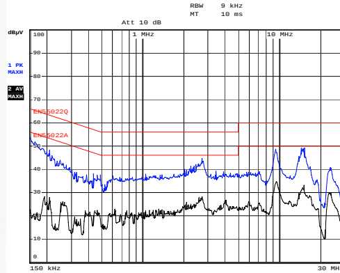
Figure 20. Conduction-Neutral at 115V AC
