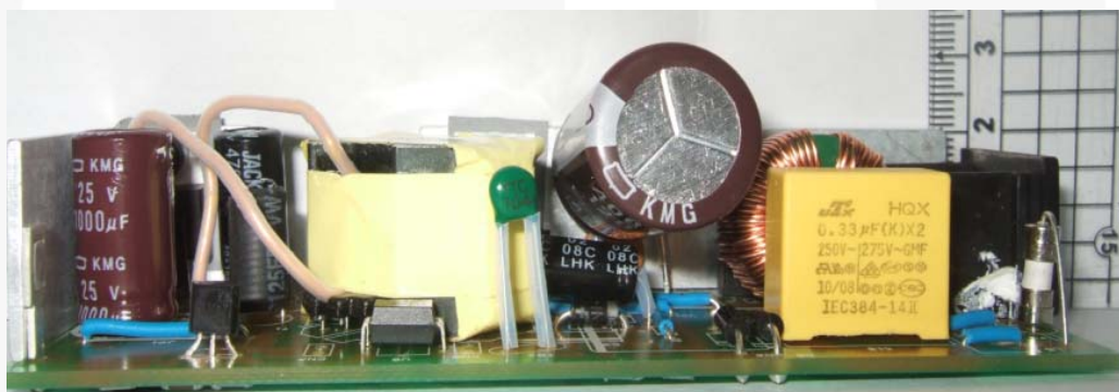
Figure 23. Side View
