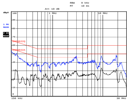
Figure 19. Conduction-Line at 230V AC
