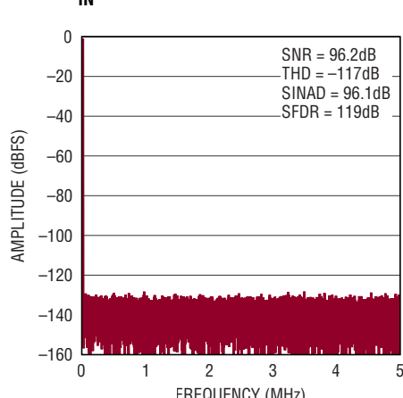
32k Point FFT f_{\text{SAMPL}} = 10\text{Mps} , f_{\text{IN}} = 2\text{kHz}
