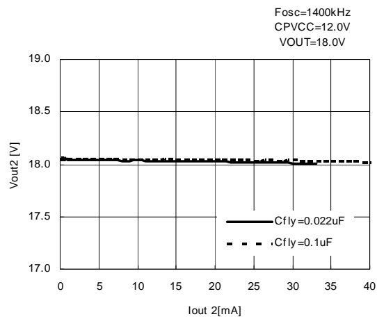
R1290K102A
