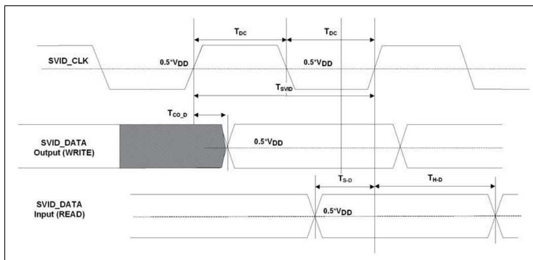
Figure 33-17.SVID Timing Diagram
