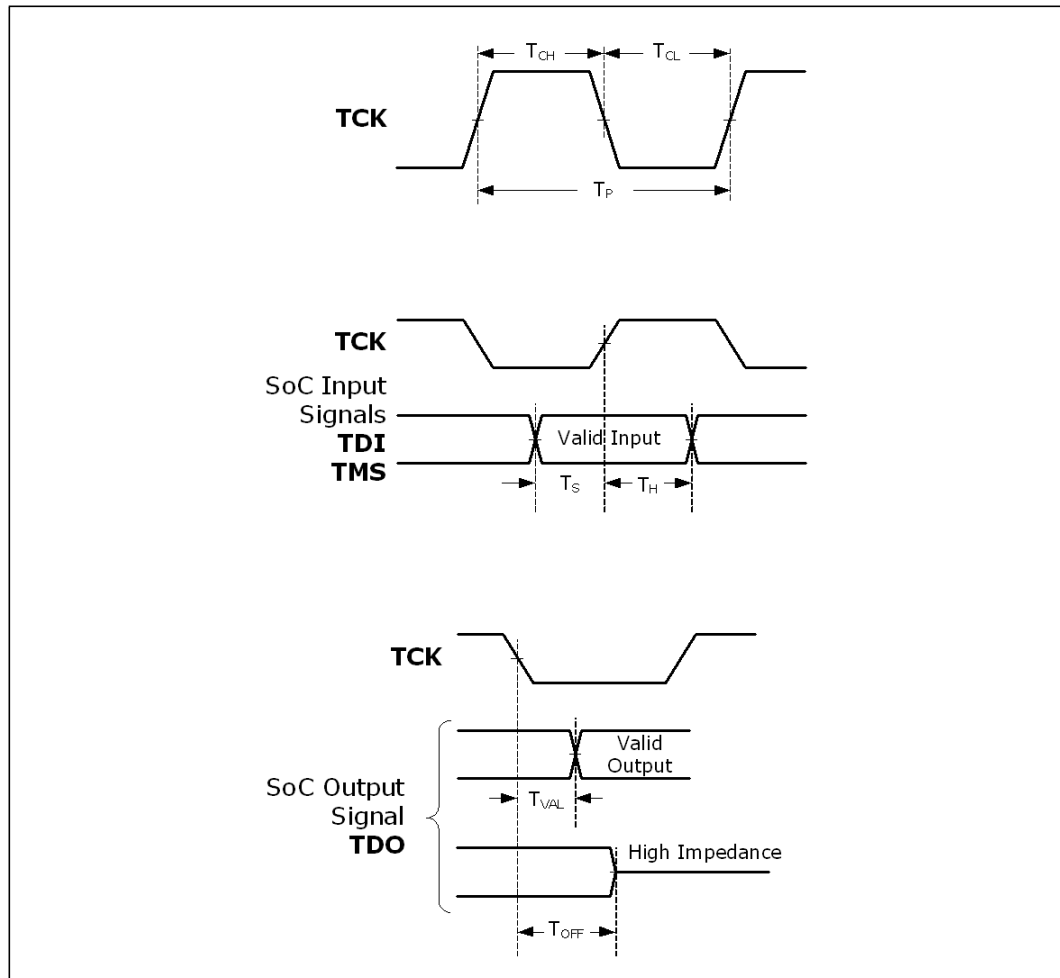
Figure 33-18.JTAG Timing Diagram
