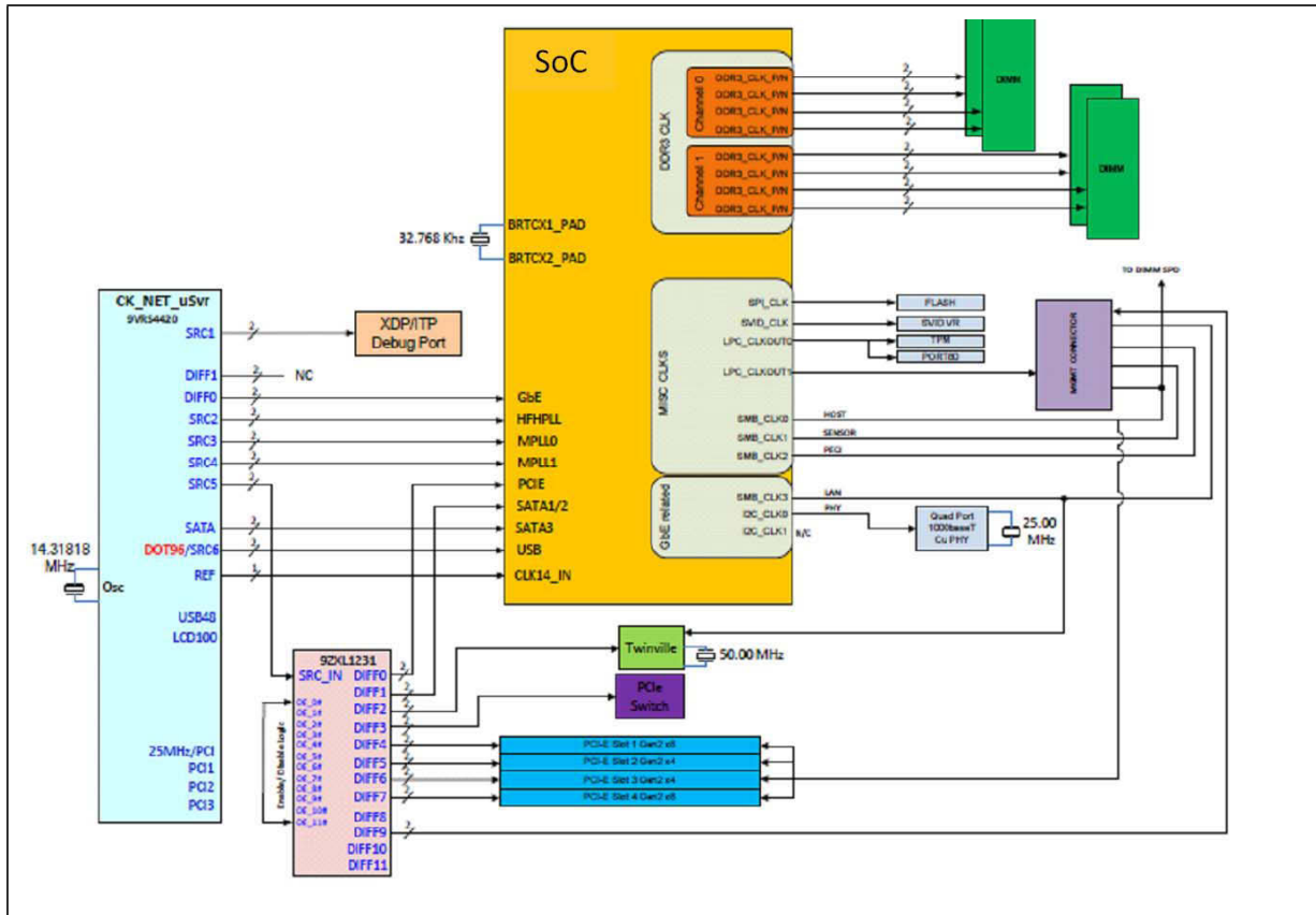
Figure 5-1. Clock Architecture
