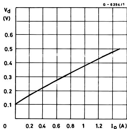
Figure 6. Dropout voltage vs. output current
