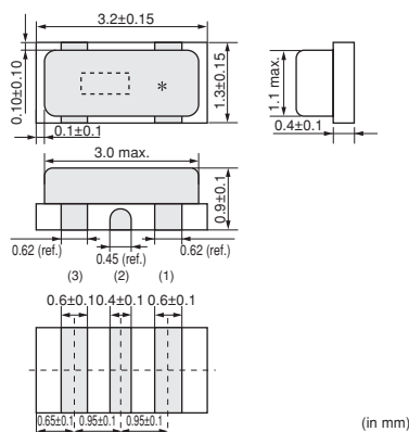
CSTCE_V 14.00-20.00MHz
