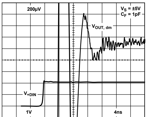
Figure 25. Settling Time
