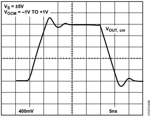
Figure 36. V_{OCM} Transient Response
