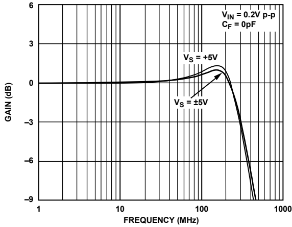
Figure 5. Small Signal Frequency Response
