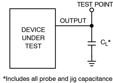
Figure 5. Test Circuit
