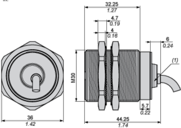
(1) LED
