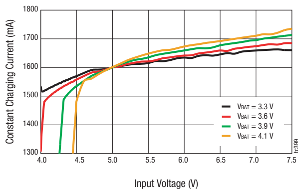
Figure 11. Constant Charging Current vs Input Voltage ( R_{SET} = 866 \Omega )
