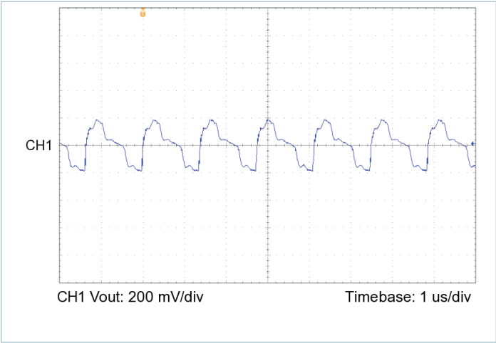
Figure 16 — Output voltage ripple, V_{IN} = 30\text{ V} , V_{OUT} = 28.0\text{ V} , C_{OUT\_EXT} = 1000\ \mu\text{F} , R_{LOAD} = 4.828\ \Omega
