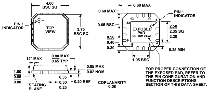
Figure 64. 16-Lead Lead Frame Chip Scale Package [LFCSP_VQ] 4 mm × 4 mm Body, Very Thin Quad (CP-16-10)
