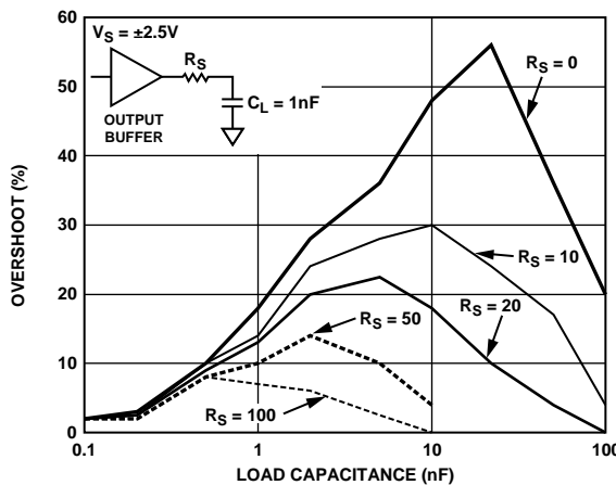
Figure 57. Positive Overshoot Graph vs. C_L
