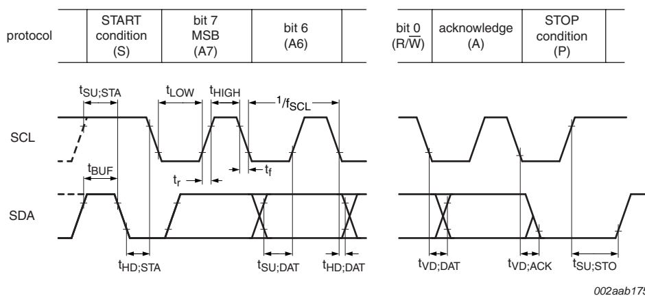
Fig 38. I 2 C-bus timing diagram
