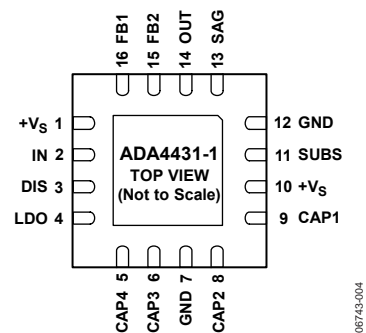
Figure 4. Pin Configuration
