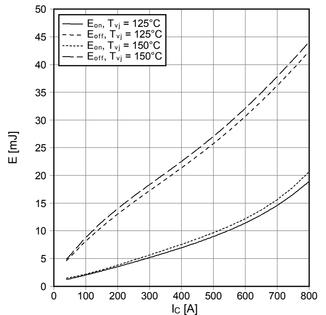
Schaltverluste IGBT-Wechselr. (typisch) switching losses IGBT-inverter (typical) E_{on} = f(I_c) , E_{off} = f(I_c) V_{GE} = \pm 15\text{ V} , R_{Gon} = 1.5\ \Omega , R_{Goff} = 0.82\ \Omega , V_{CE} = 300\text{ V}
