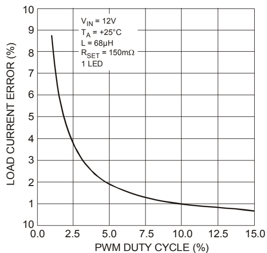
Figure 35. Low Duty Cycle PWM Dimming at 500Hz
