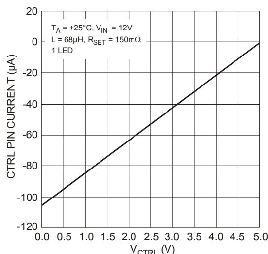
Figure 5. I_{CTRL} vs. V_{CTRL}
