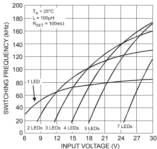
Figure 31. Switching Frequency vs. Input Voltage
