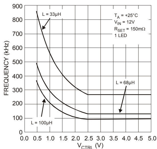
Figure 3. Switching Frequency vs. V_{CTRL}
