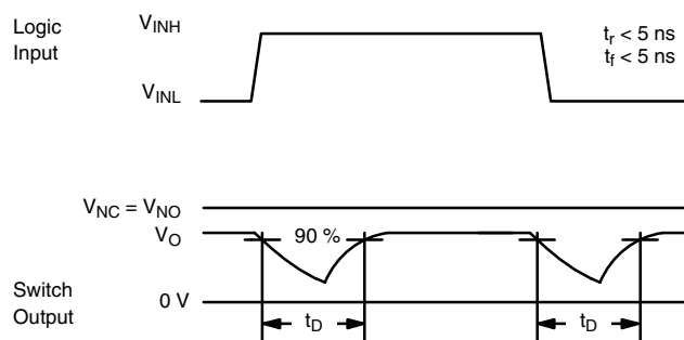
Figure 3. Break-Before-Make (DG419L)
