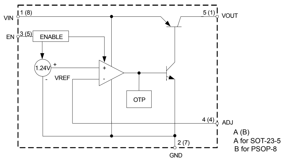
Adjustable Output Voltage
