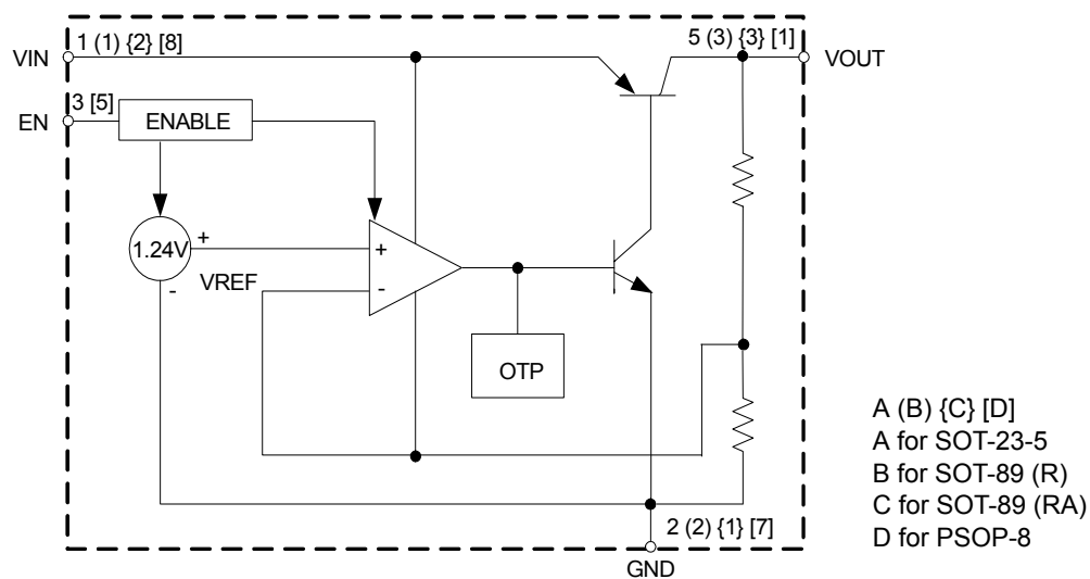
Fixed Output Voltage
