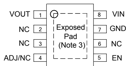
MP Package (PSOP-8)
