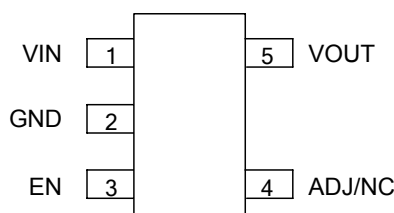
K Package (SOT-23-5)
