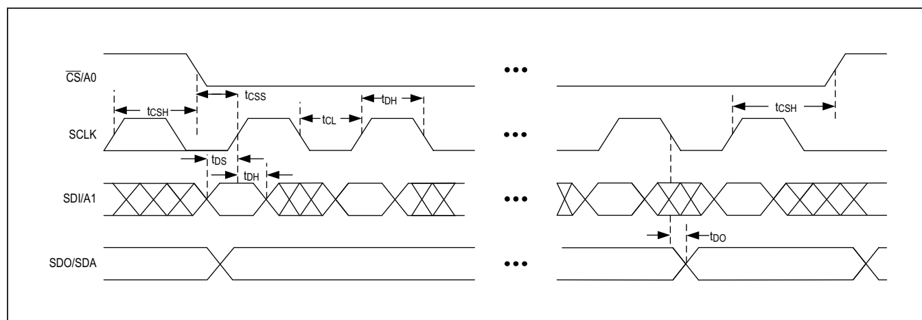
Figure 6. SPI Timing
