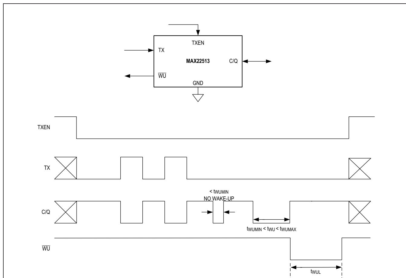
Figure 5. Wake-Up Timing
