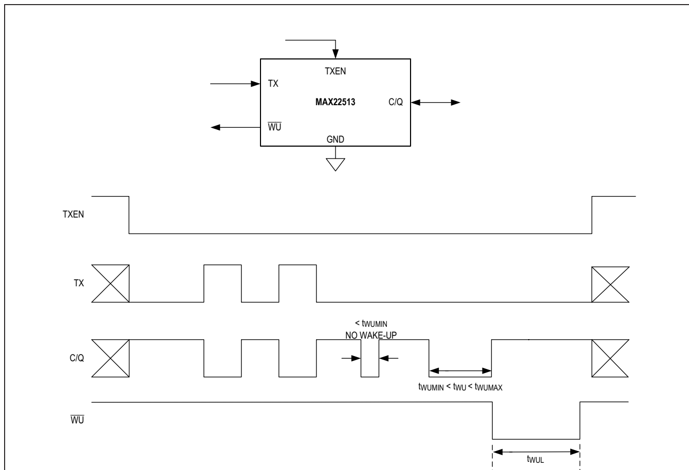
Figure 5. Wake-Up Timing
