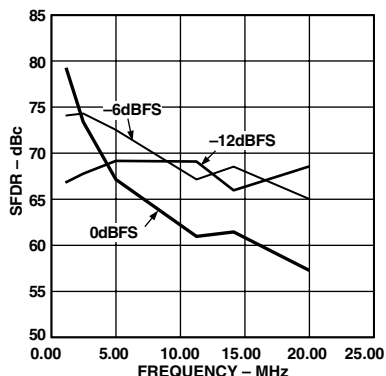
Figure 24. SFDR vs. f_{OUT} @ 50 MSPS
