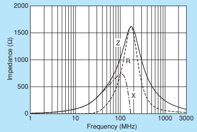
BLM18BD102SN1
