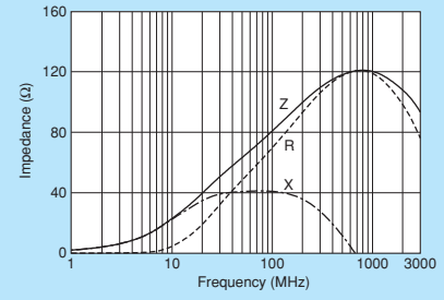
BLM03PX800SN1
