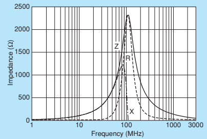
BLM18BD222SN1
