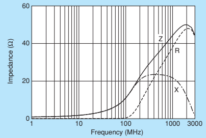
BLM18BB100SN1
