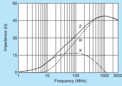
BLM03PX330SN1
