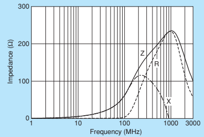
BLM18BB600SN1
