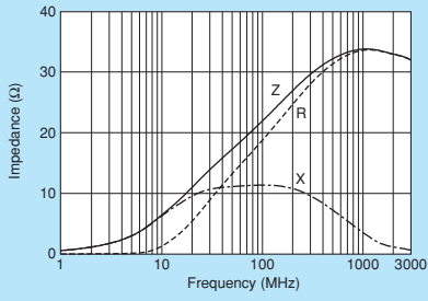
BLM03PX220SN1
