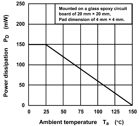
Fig. 7.4 P_D - T_a
