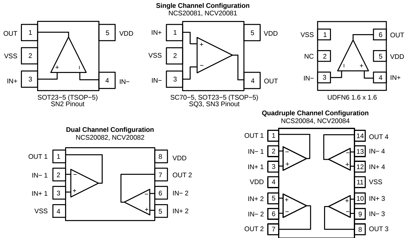
Figure 1. Pin Connections
