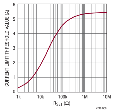
Current Limit Adjustment ( I_{OUT} vs R_{SET} )
