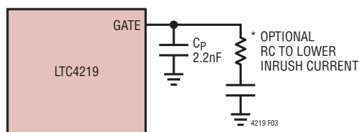
Figure 3. Compensation for Small C_{\text{LOAD}}
