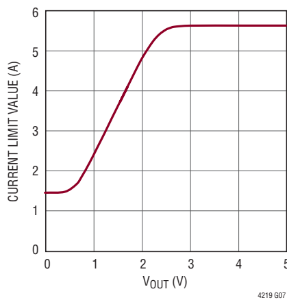
Current Limit Threshold Foldback, LTC4219-5
