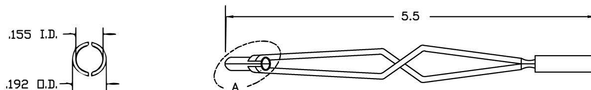
VIEW A
