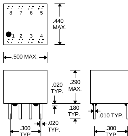
MDU28C-xxM (Military DIP)
