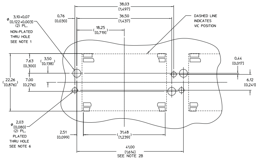
Figure 14 — Hole location for push pin heat sink relative to V-I Chip™ module
